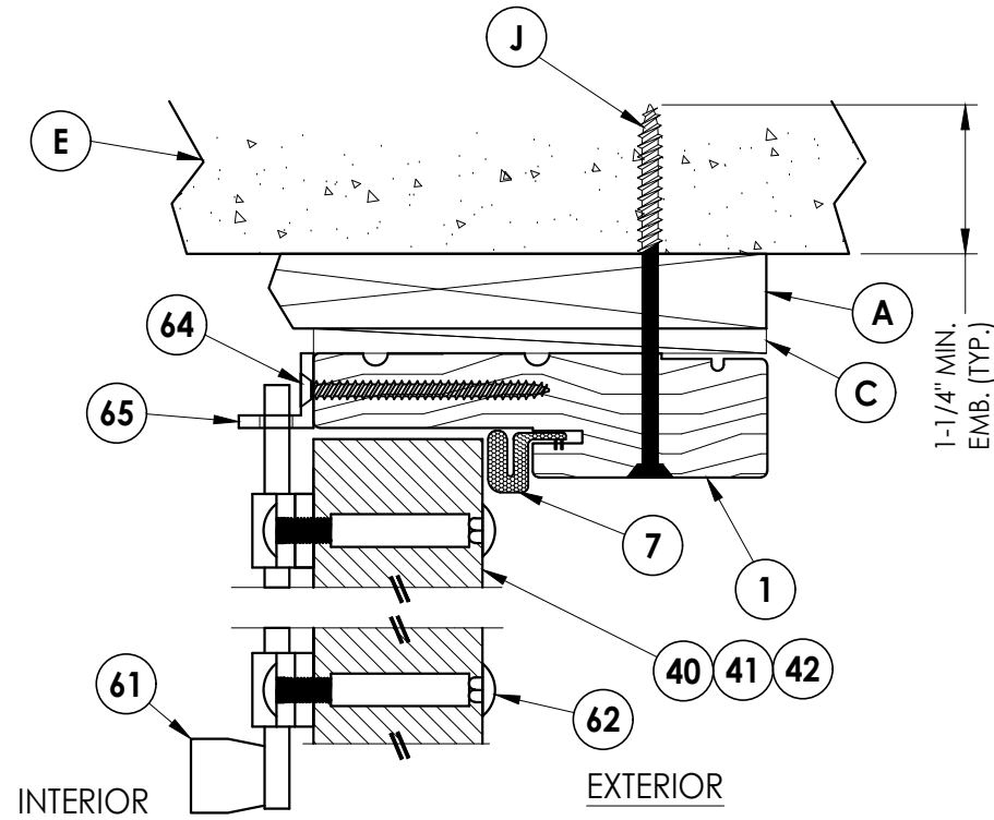
2 9 VERTICAL CROSS SECTION Surface Bolt - Inswing shown Shown w/ 1X sub-buck
