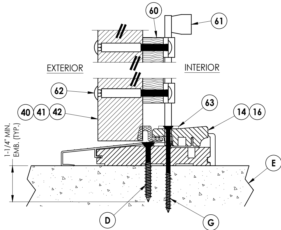
3 9 VERTICAL CROSS SECTION Surface Bolt - Outswing Threshold
