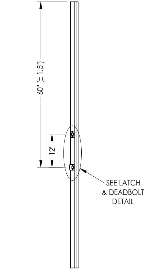
ASTRAGAL Latch & Deadbolt
