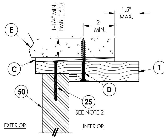
3 VERTICAL CROSS SECTION 7 Shown Direct to Masonry Outswing only w/ 6-9/16" jamb
