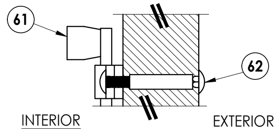
2 9 VERTICAL CROSS SECTION Surface Bolt - Inswing shown Shown w/ 1X sub-buck
